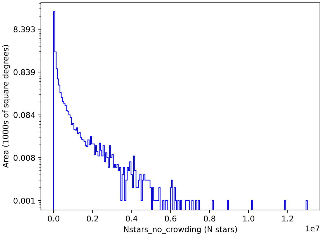
ddf_loaded_half_fl1_v3.4_10yrs g: Nstars_no_crowding
