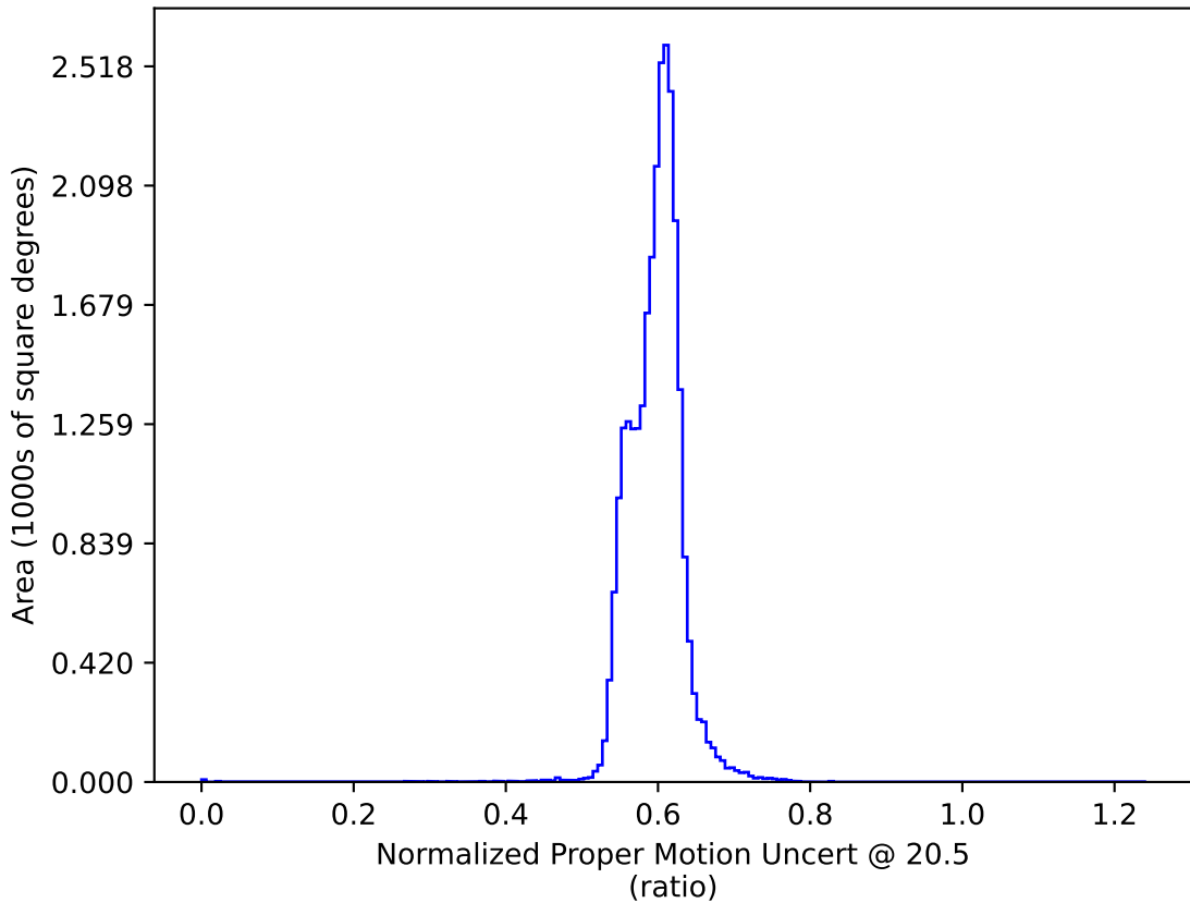
ddf_loaded_half_fl1_v3.4_10yrs : Normalized Proper Motion Uncert @ 20.5
