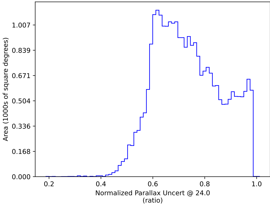
ddf_loaded_half_fl1_v3.4_10yrs : Normalized Parallax Uncert @ 24.0
