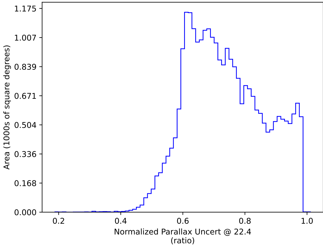
ddf_loaded_half_fl1_v3.4_10yrs : Normalized Parallax Uncert @ 22.4
