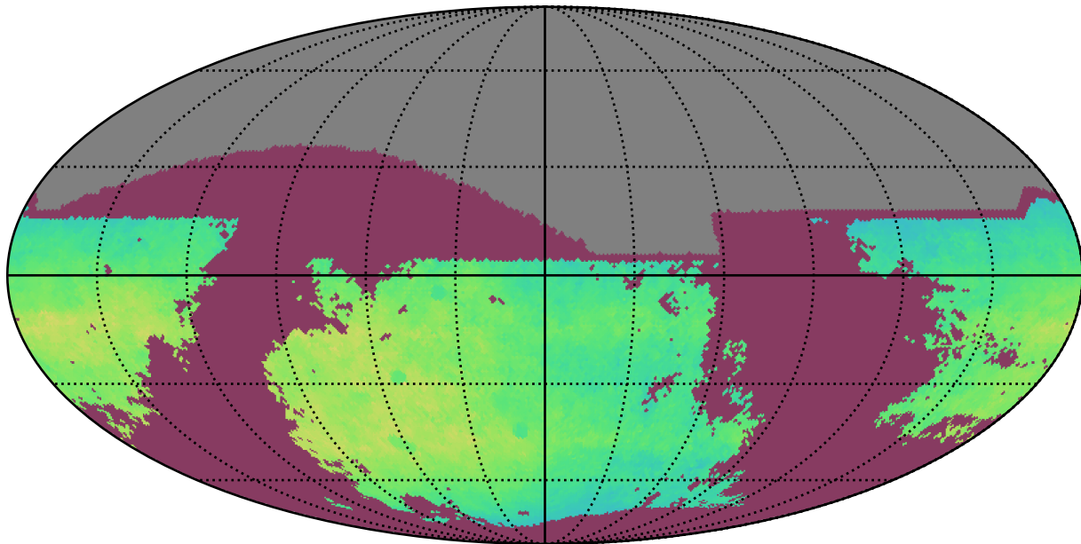
ddf_loaded_half_fl1_v3.4_10yrs i: NgalScale
