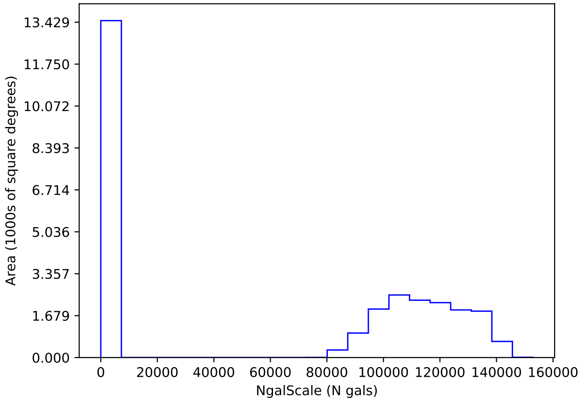
ddf_loaded_half_fl1_v3.4_10yrs i: NgalScale
