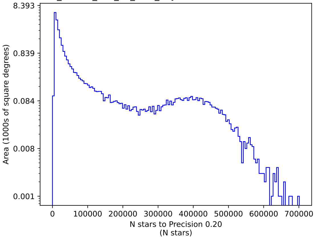
ddf_loaded_half_fl1_v3.4_10yrs z: N stars to Precision 0.20
