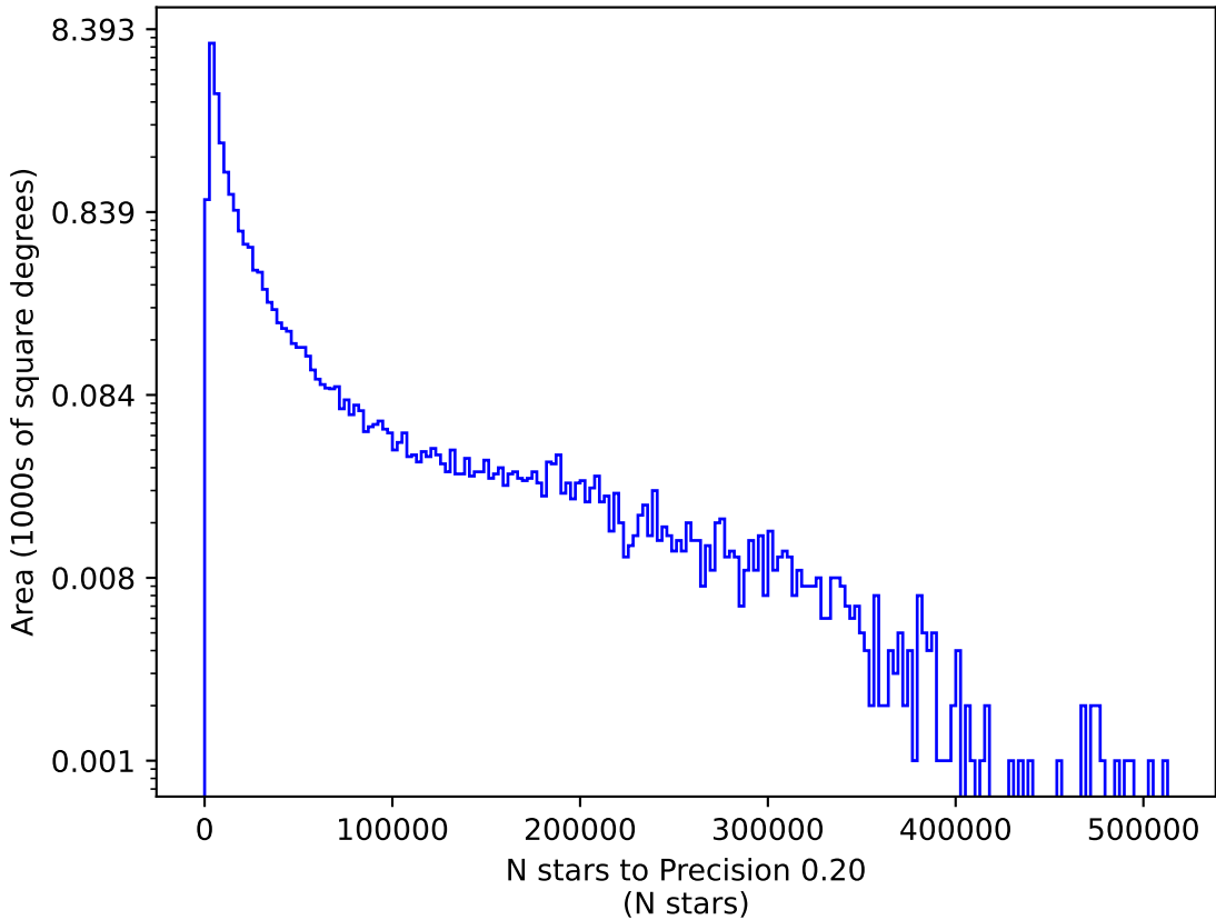
ddf_loaded_half_fl1_v3.4_10yrs u: N stars to Precision 0.20
