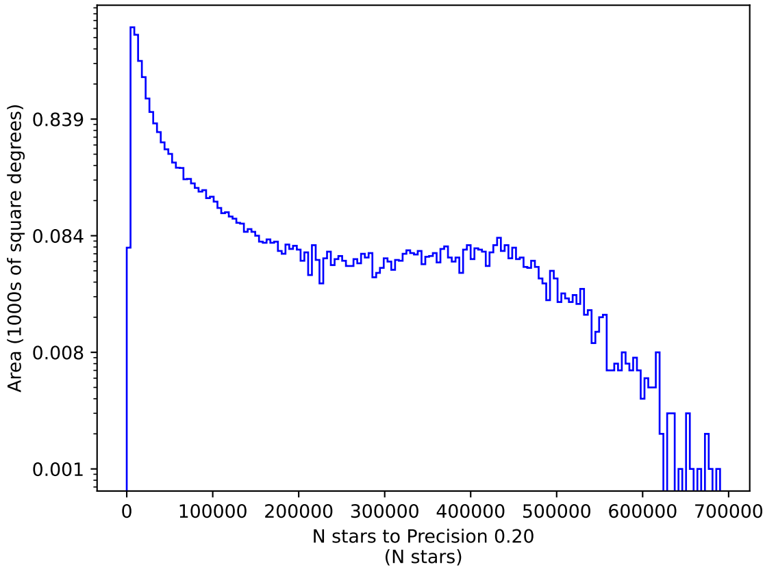
ddf_loaded_half_fl1_v3.4_10yrs r: N stars to Precision 0.20
