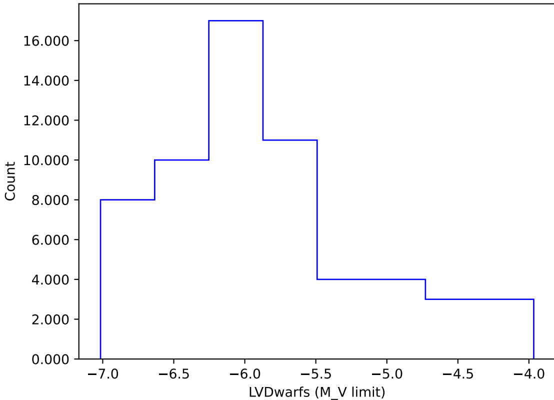
ddf_loaded_half_fl1_v3.4_10yrs gi: LVDwarfs
