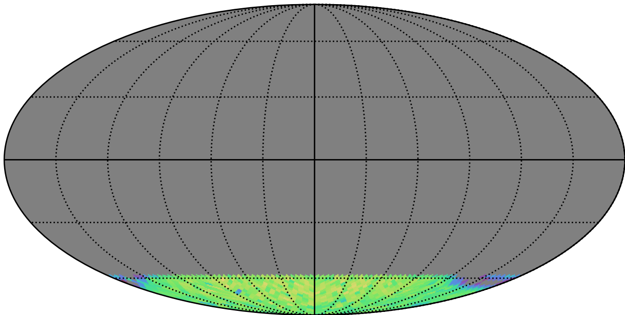
ddf_loaded_half_fl1_v3.4_10yrs gi SCP: LVDwarfs
