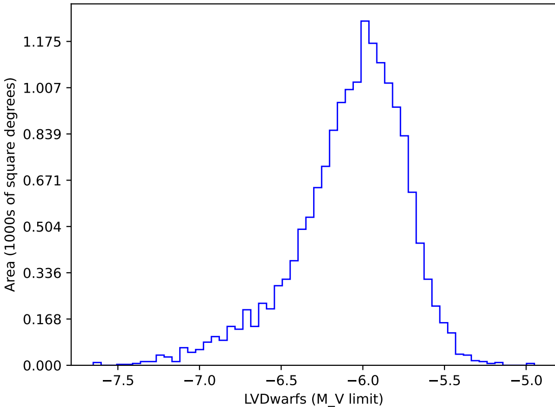
ddf_loaded_half_fl1_v3.4_10yrs gi: LVDwarfs
