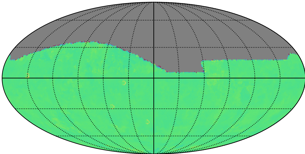
ddf_loaded_half_fl1_v3.4_10yrs z: Kuiper rotTelPos
