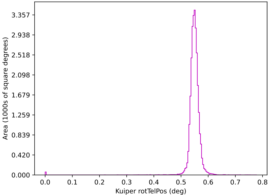
ddf_loaded_half_fl1_v3.4_10yrs z: Kuiper rotTelPos
