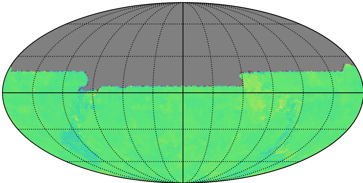
ddf_loaded_half_fl1_v3.4_10yrs u: Kuiper rotTelPos
