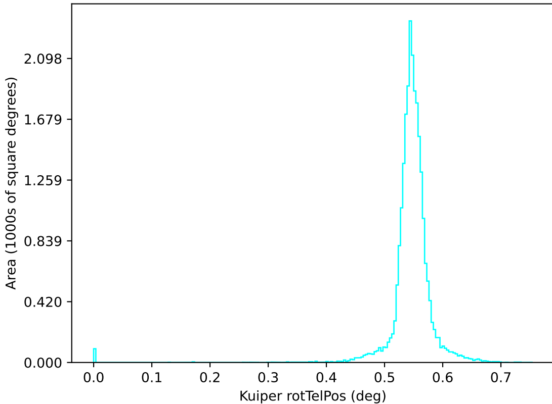
ddf_loaded_half_fl1_v3.4_10yrs u: Kuiper rotTelPos
