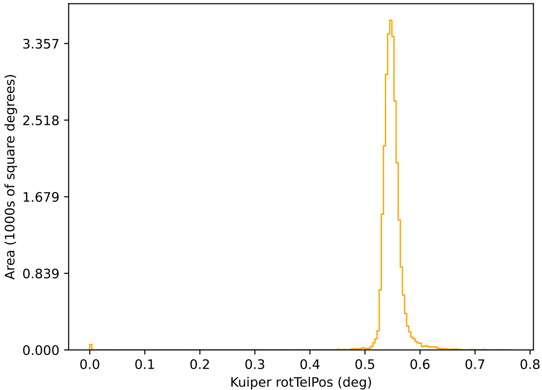
ddf_loaded_half_fl1_v3.4_10yrs r: Kuiper rotTelPos
