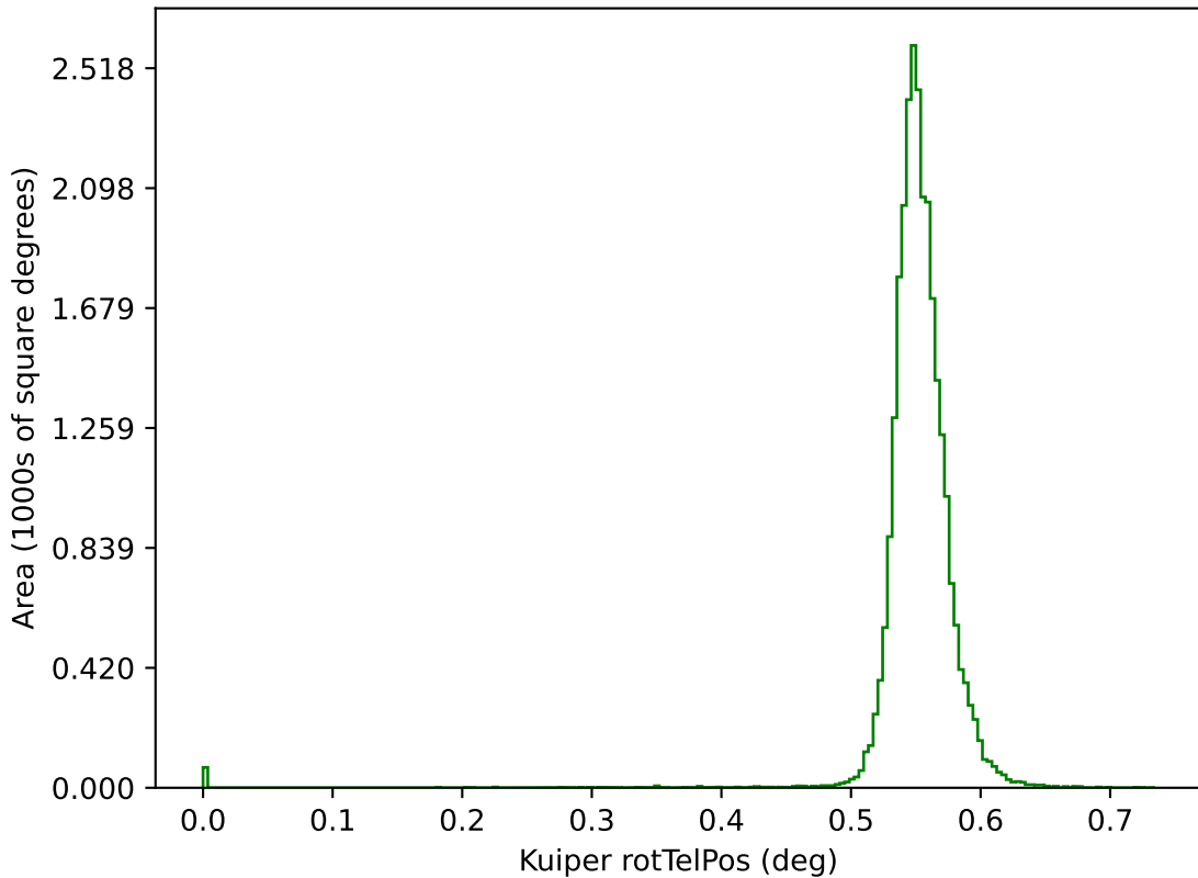
ddf_loaded_half_fl1_v3.4_10yrs g: Kuiper rotTelPos
