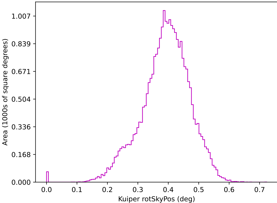
ddf_loaded_half_fl1_v3.4_10yrs z: Kuiper rotSkyPos
