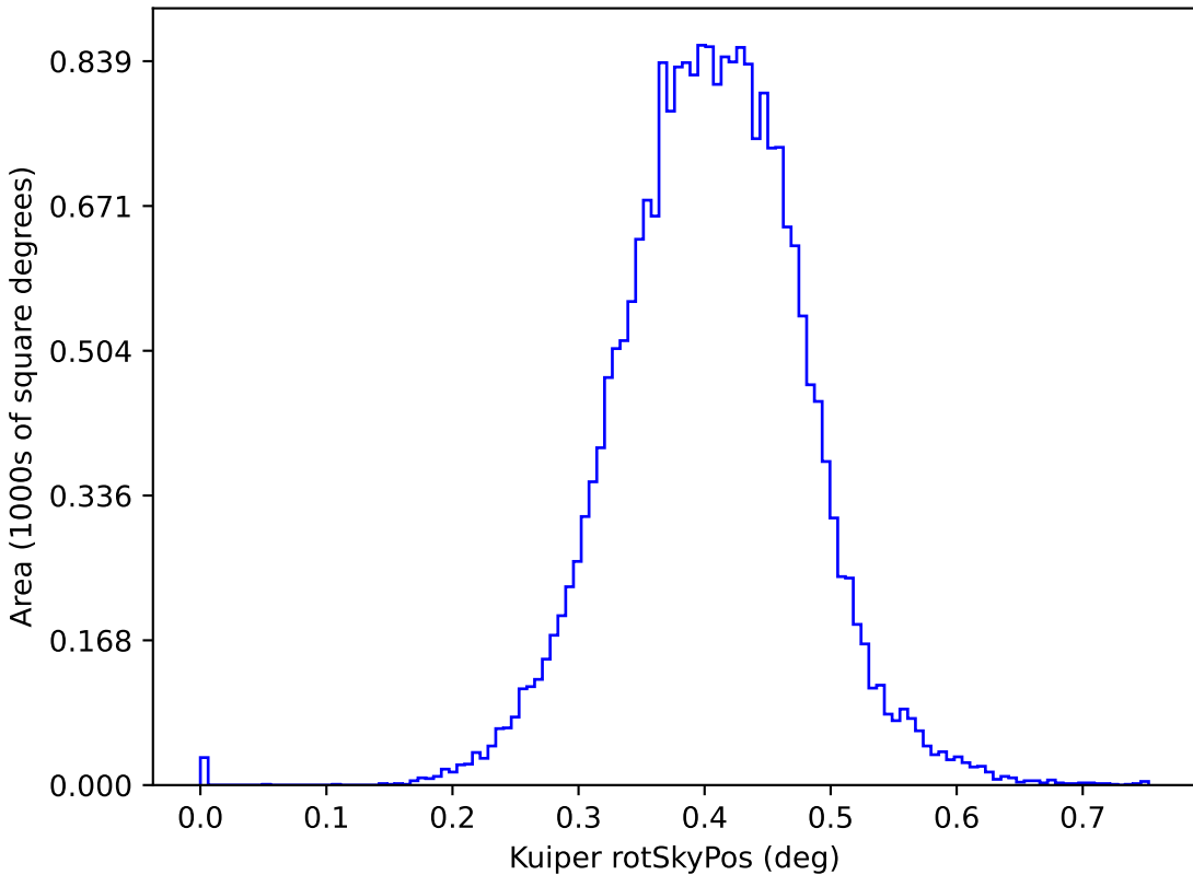
ddf_loaded_half_fl1_v3.4_10yrs y: Kuiper rotSkyPos
