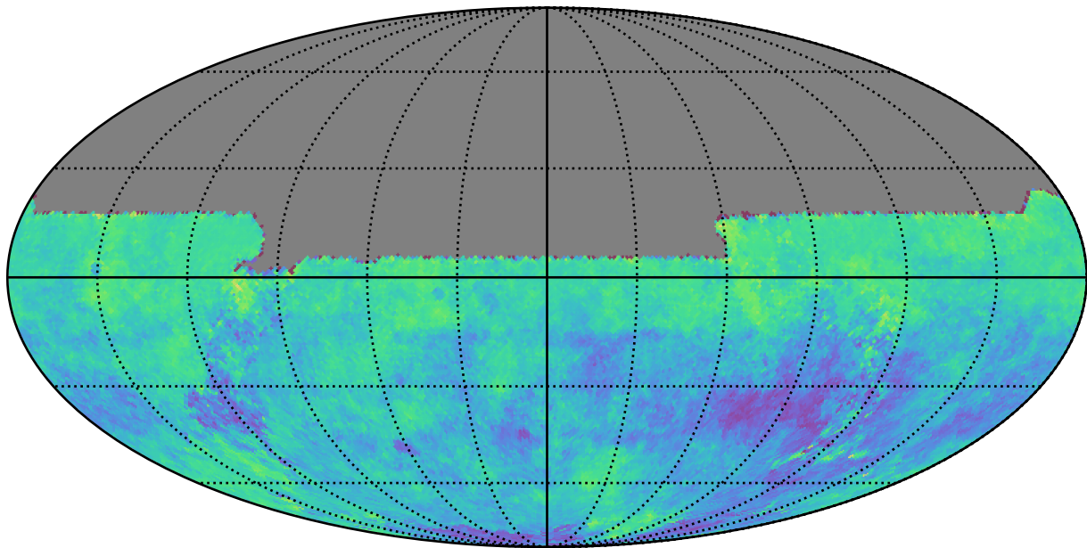
ddf_loaded_half_fl1_v3.4_10yrs u: Kuiper rotSkyPos
