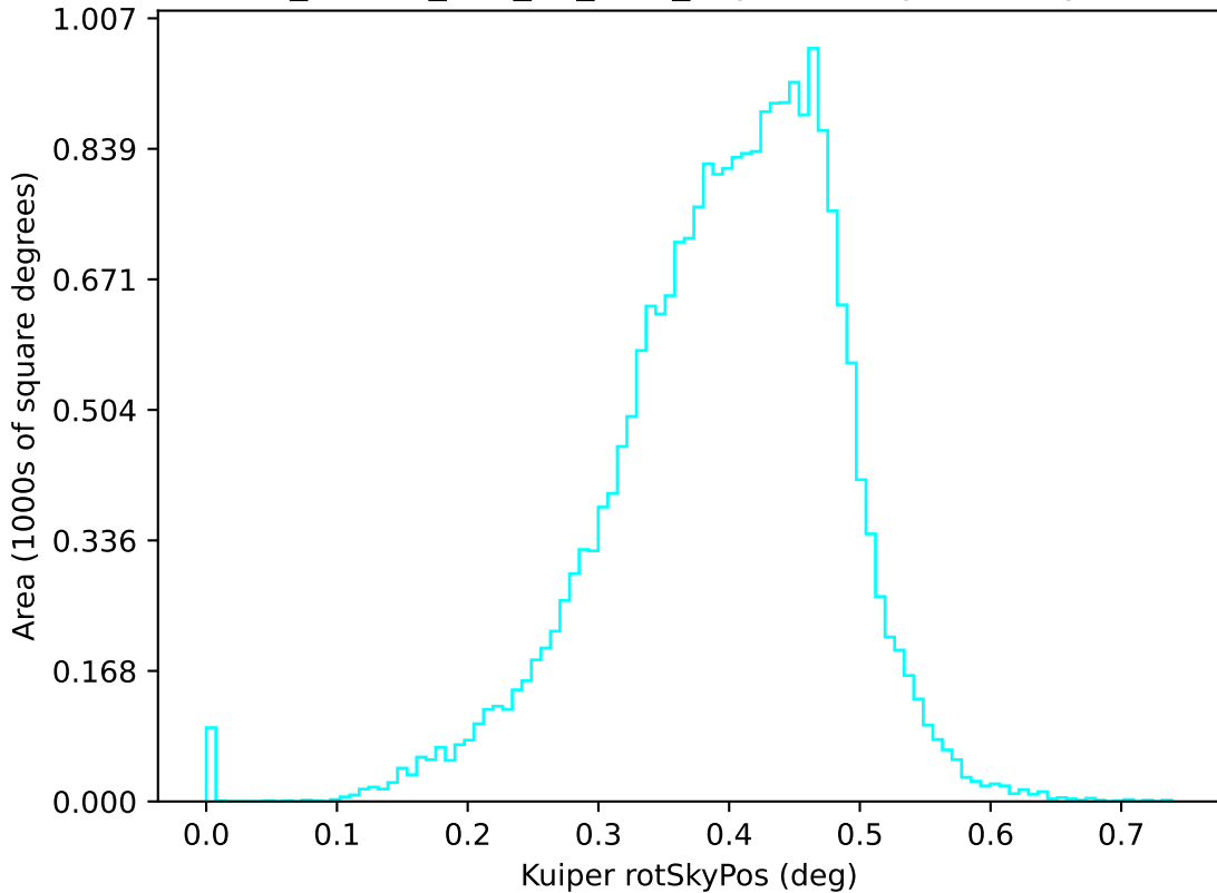
ddf_loaded_half_fl1_v3.4_10yrs u: Kuiper rotSkyPos
