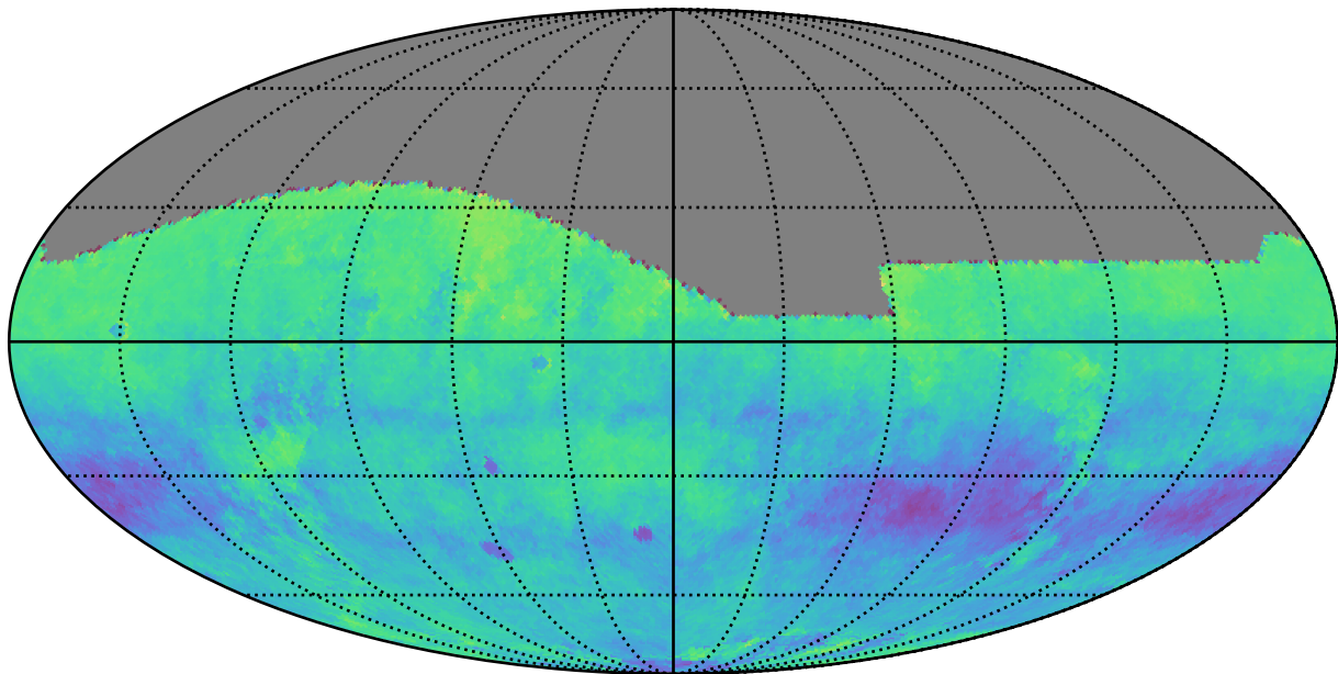
ddf_loaded_half_fl1_v3.4_10yrs r: Kuiper rotSkyPos
