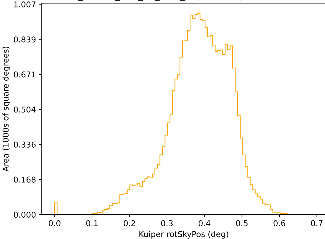
ddf_loaded_half_fl1_v3.4_10yrs r: Kuiper rotSkyPos
