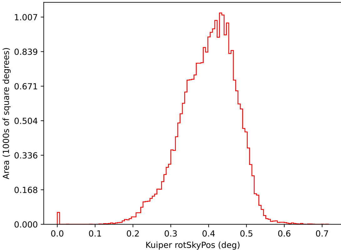
ddf_loaded_half_fl1_v3.4_10yrs i: Kuiper rotSkyPos
