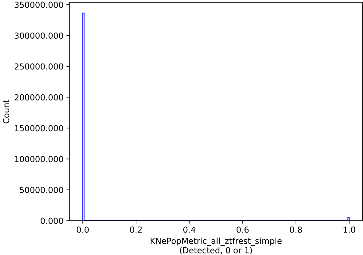
ddf_loaded_half_fl1_v3.4_10yrs all models: KNePopMetric_all_ztfrest_simple
