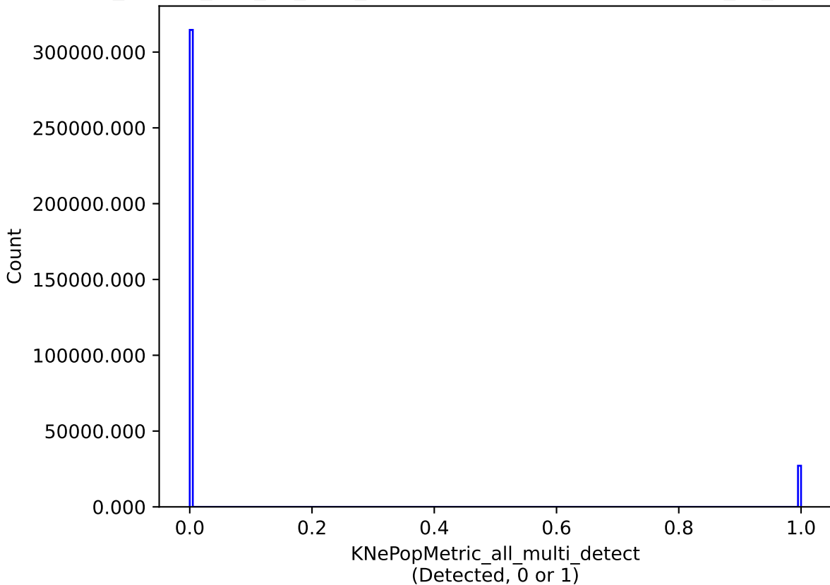
ddf_loaded_half_fl1_v3.4_10yrs all models: KNePopMetric_all_multi_detect
