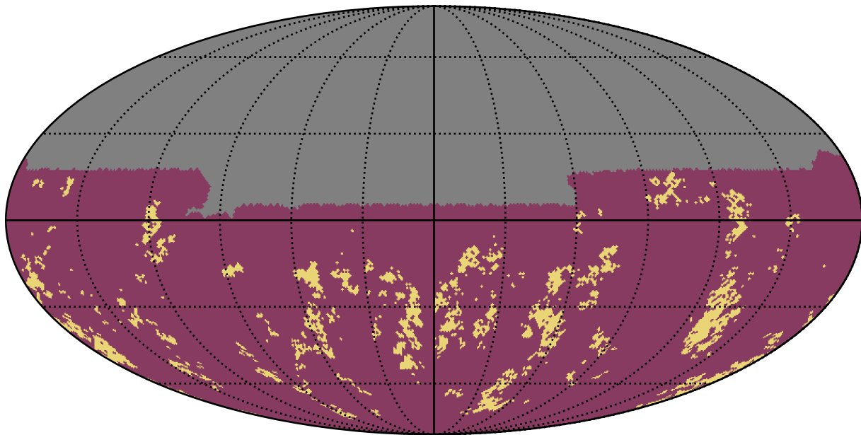
ddf_loaded_half_fl1_v3.4_10yrs u band: Gaps_7hr
