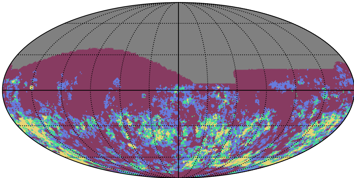
ddf_loaded_half_fl1_v3.4_10yrs i band: Gaps_7hr
