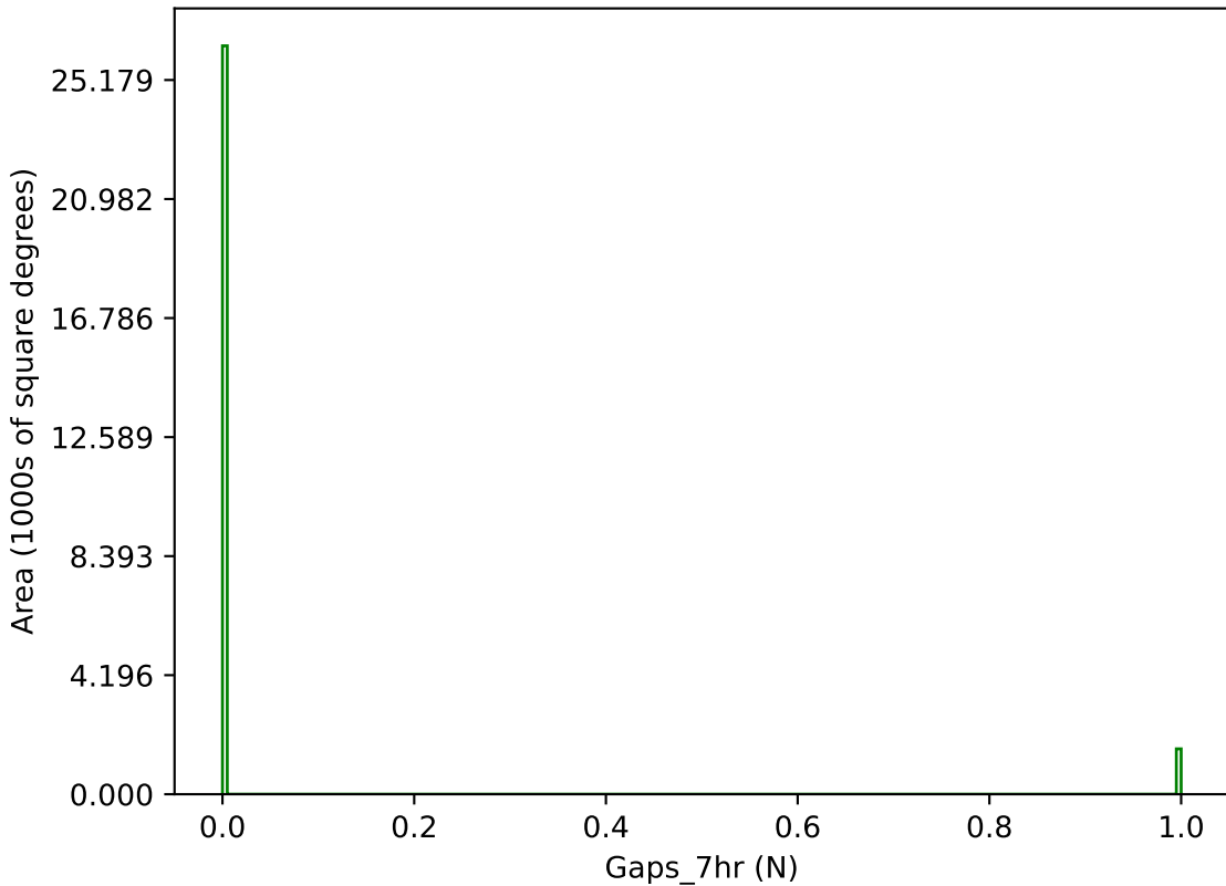
ddf_loaded_half_fl1_v3.4_10yrs g band: Gaps_7hr
