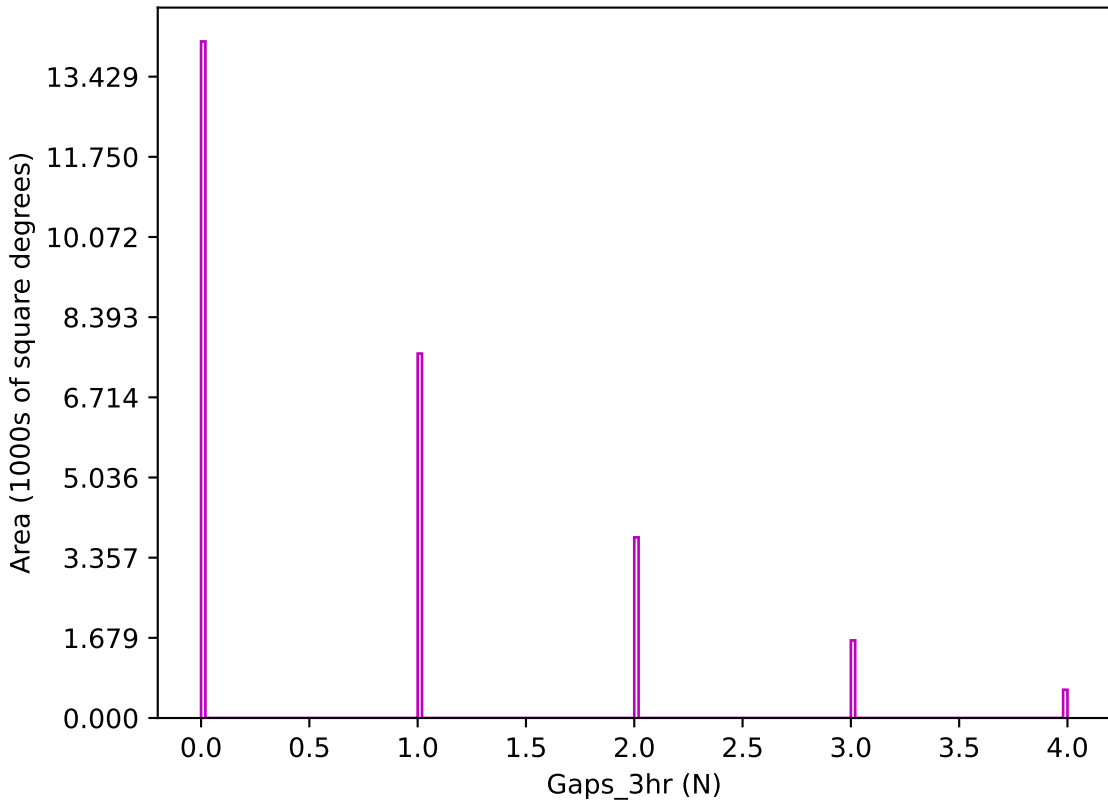
ddf_loaded_half_f11_v3.4_10yrs z band: Gaps_3hr
