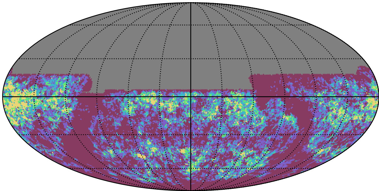
ddf_loaded_half_fl1_v3.4_10yrs y band: Gaps_3hr
