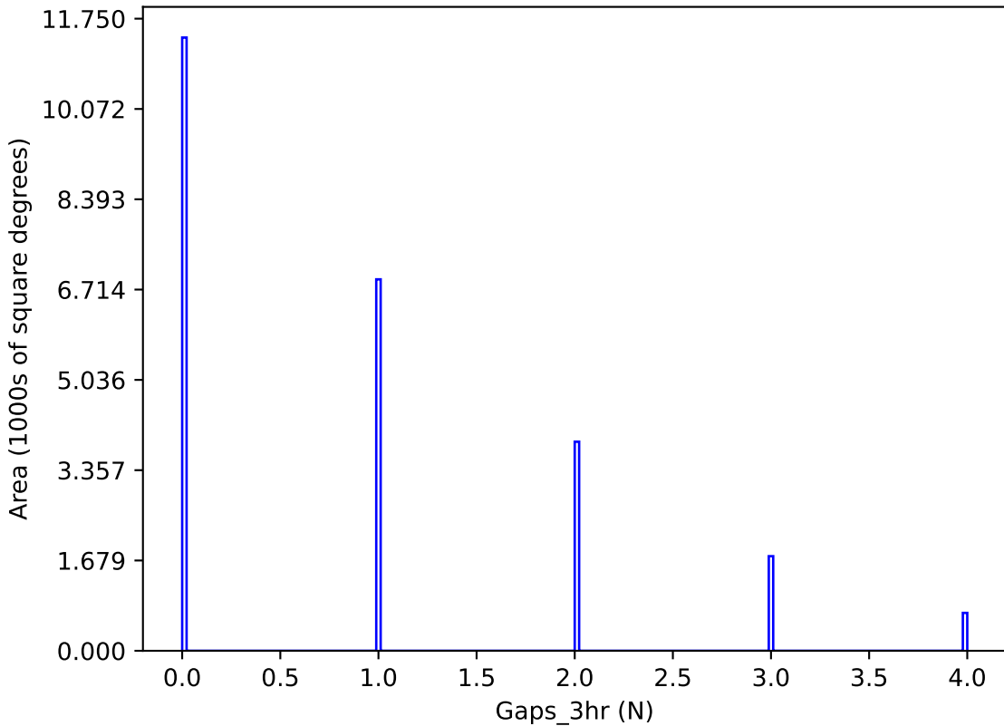
ddf_loaded_half_f11_v3.4_10yrs y band: Gaps_3hr
