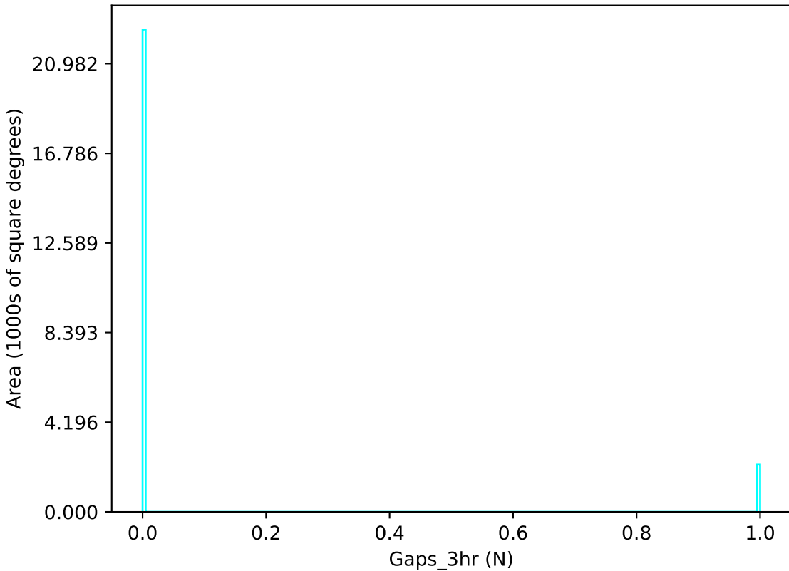
ddf_loaded_half_fl1_v3.4_10yrs u band: Gaps_3hr
