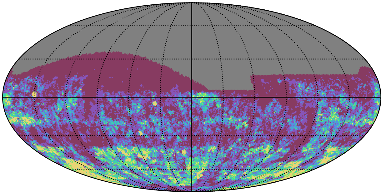
ddf_loaded_half_fl1_v3.4_10yrs r band: Gaps_3hr
