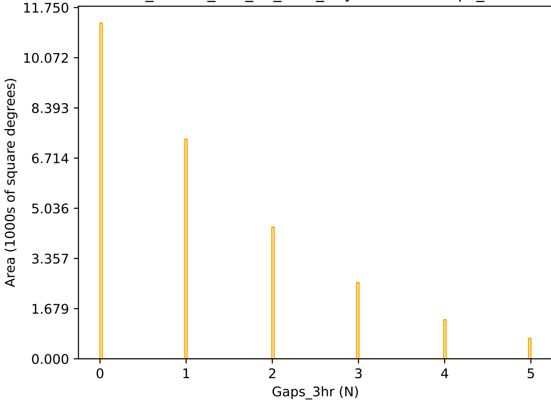
ddf_loaded_half_fl1_v3.4_10yrs r band: Gaps_3hr
