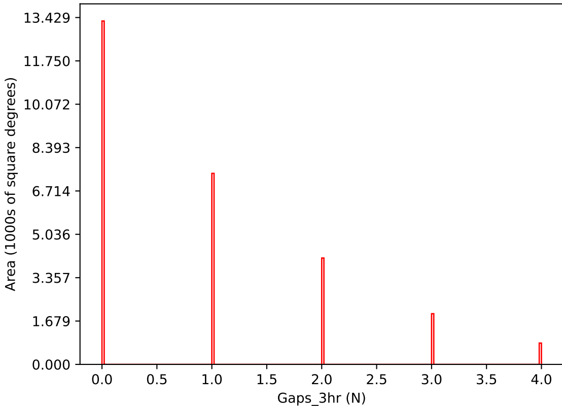
ddf_loaded_half_fl1_v3.4_10yrs i band: Gaps_3hr
