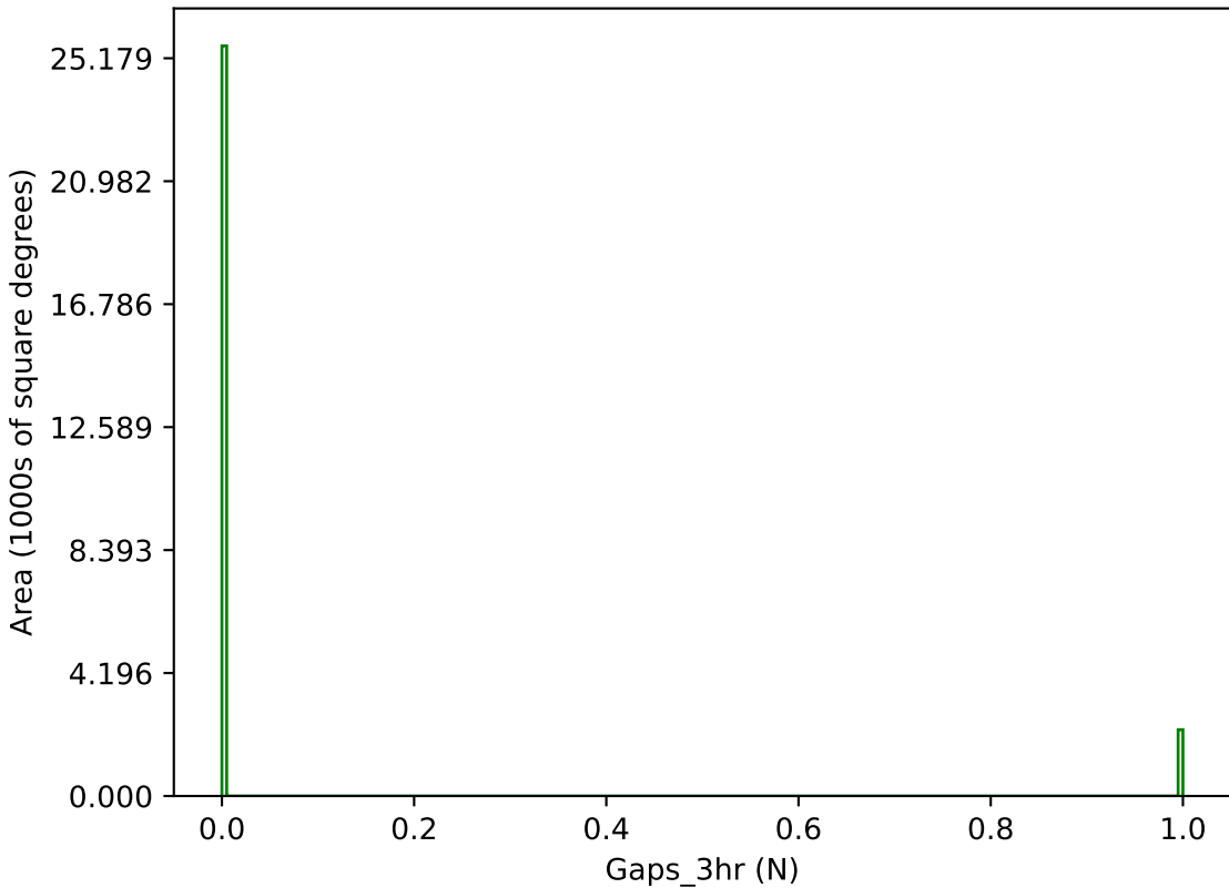
ddf_loaded_half_fl1_v3.4_10yrs g band: Gaps_3hr
