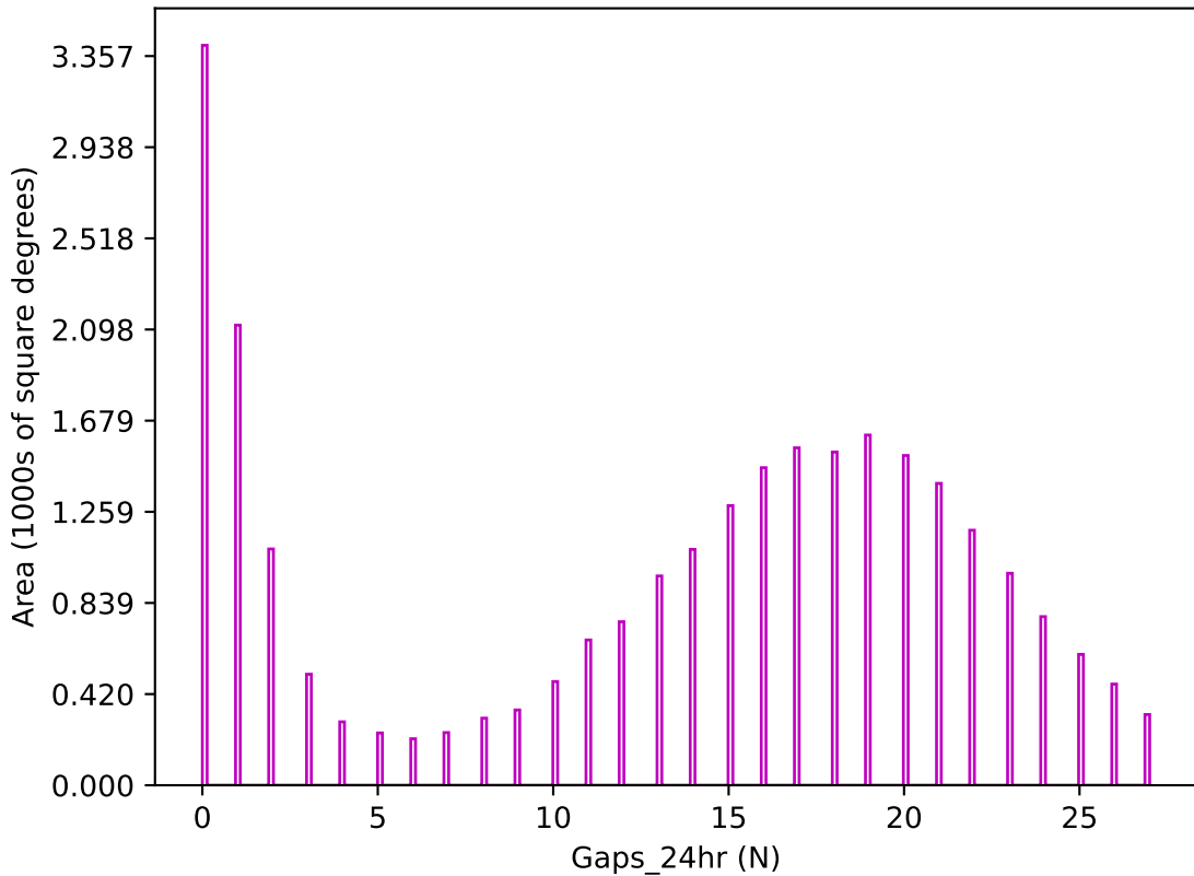
ddf_loaded_half_fl1_v3.4_10yrs z band: Gaps_24hr
