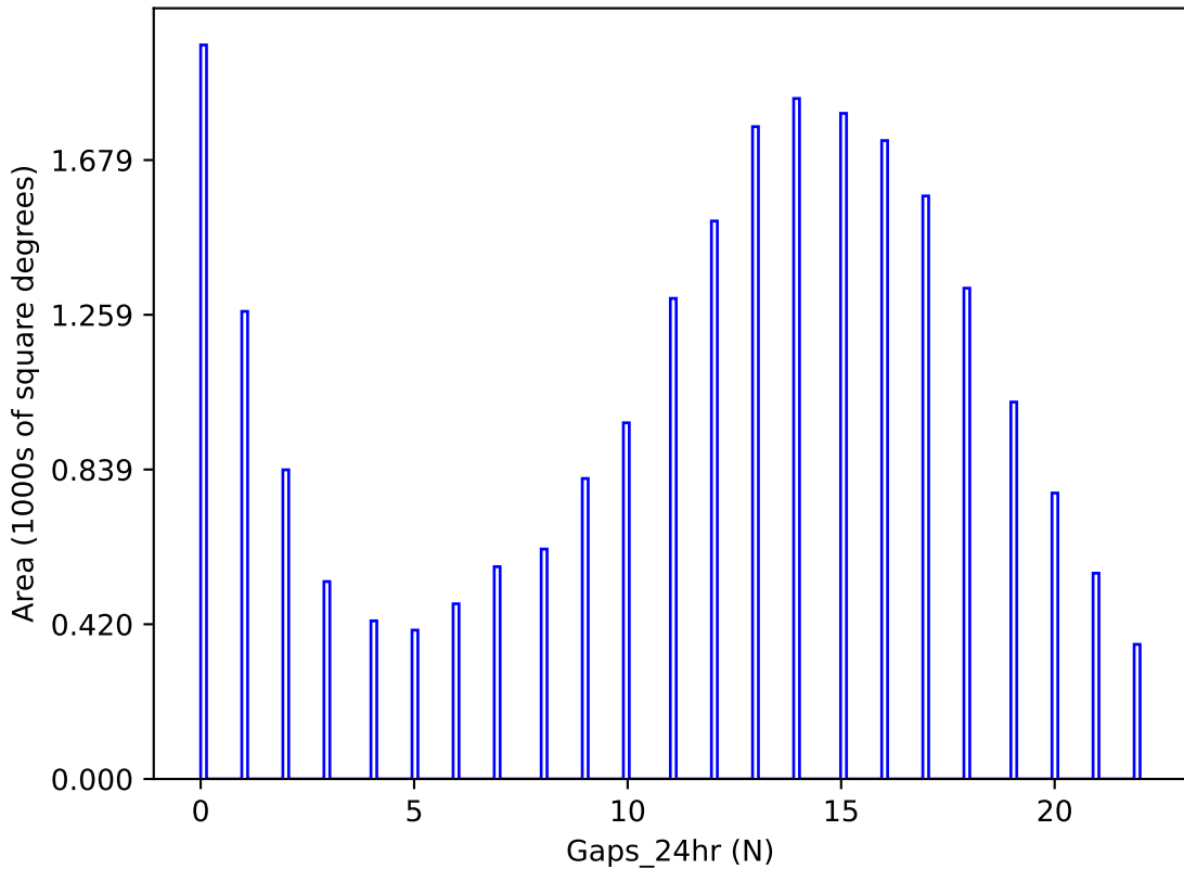
ddf_loaded_half_fl1_v3.4_10yrs y band: Gaps_24hr
