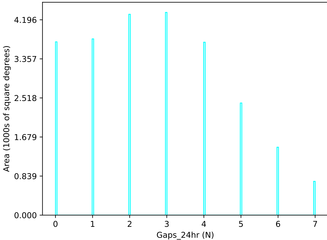
ddf_loaded_half_fl1_v3.4_10yrs u band: Gaps_24hr
