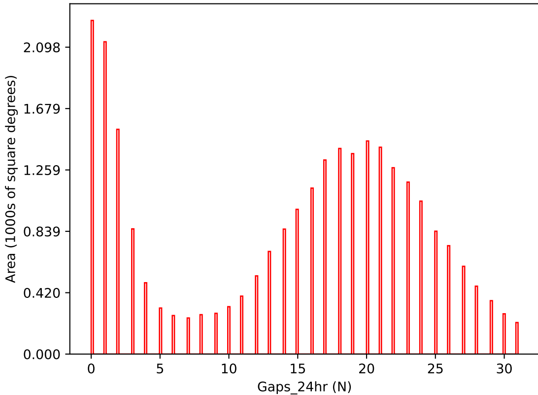
ddf_loaded_half_fl1_v3.4_10yrs i band: Gaps_24hr
