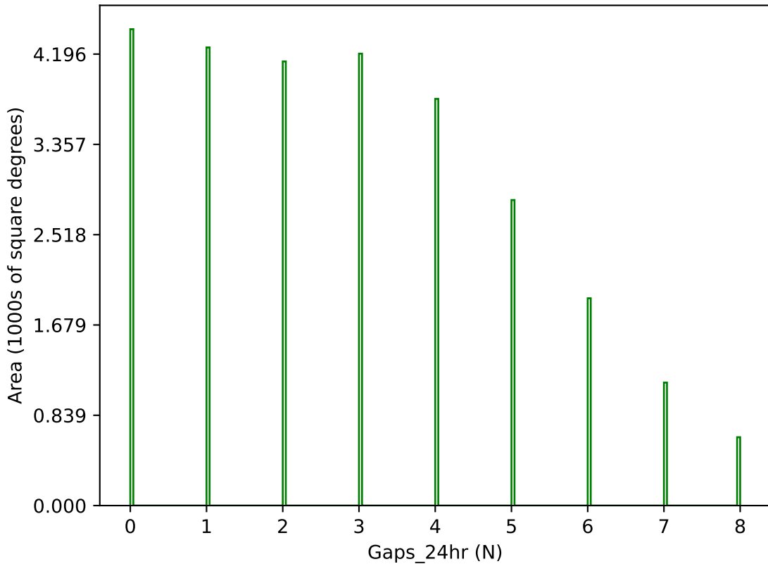
ddf_loaded_half_fl1_v3.4_10yrs g band: Gaps_24hr
