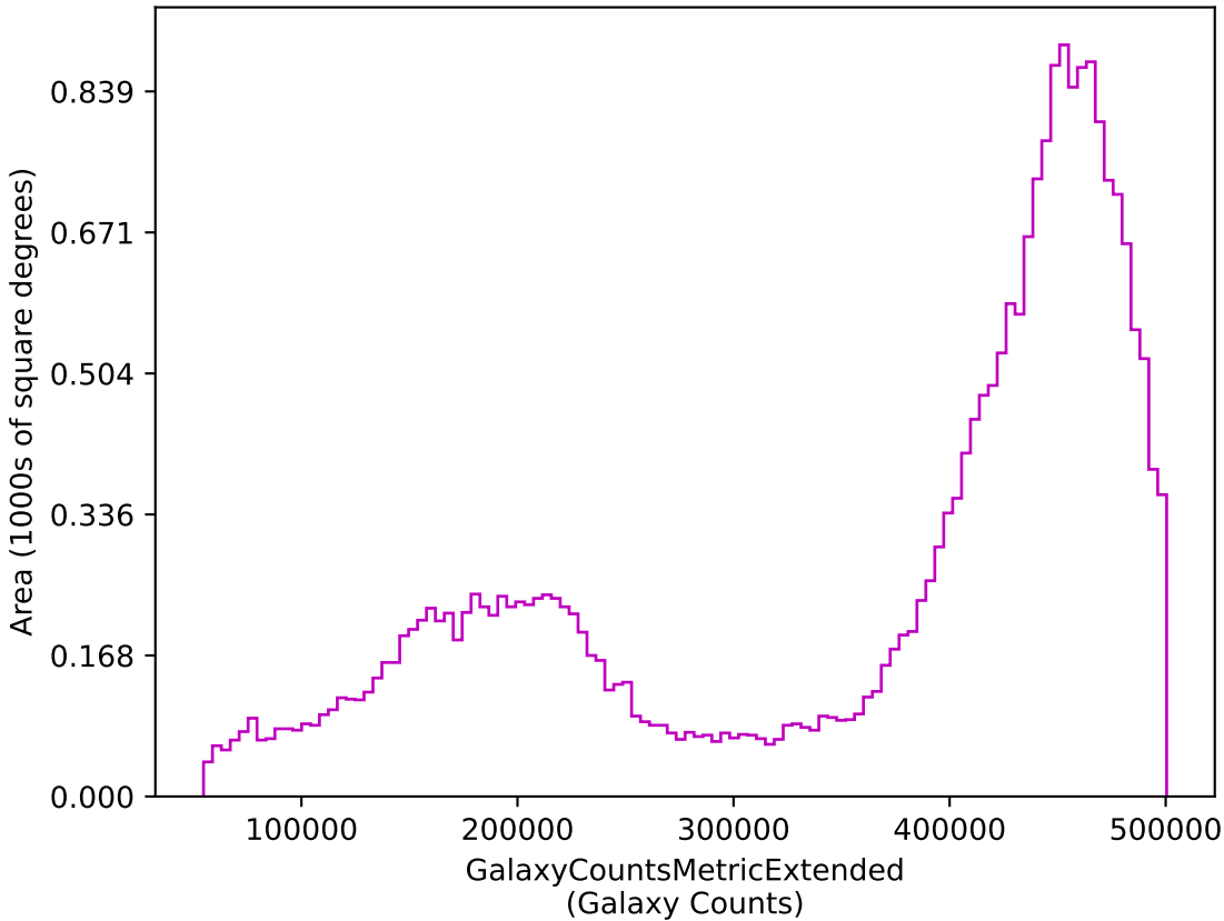
ddf_loaded_half_fl1_v3.4_10yrs z: GalaxyCountsMetricExtended
