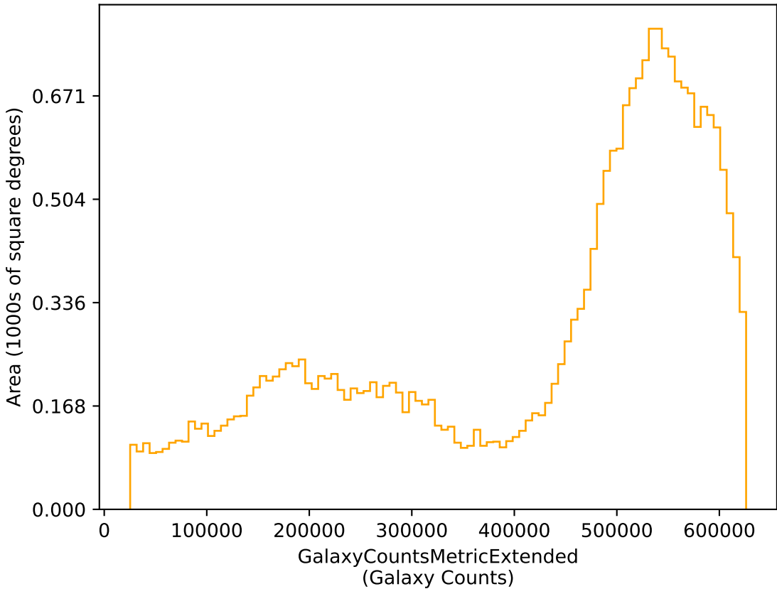
ddf_loaded_half_fl1_v3.4_10yrs r: GalaxyCountsMetricExtended
