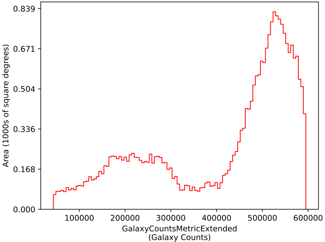
ddf_loaded_half_fl1_v3.4_10yrs i: GalaxyCountsMetricExtended
