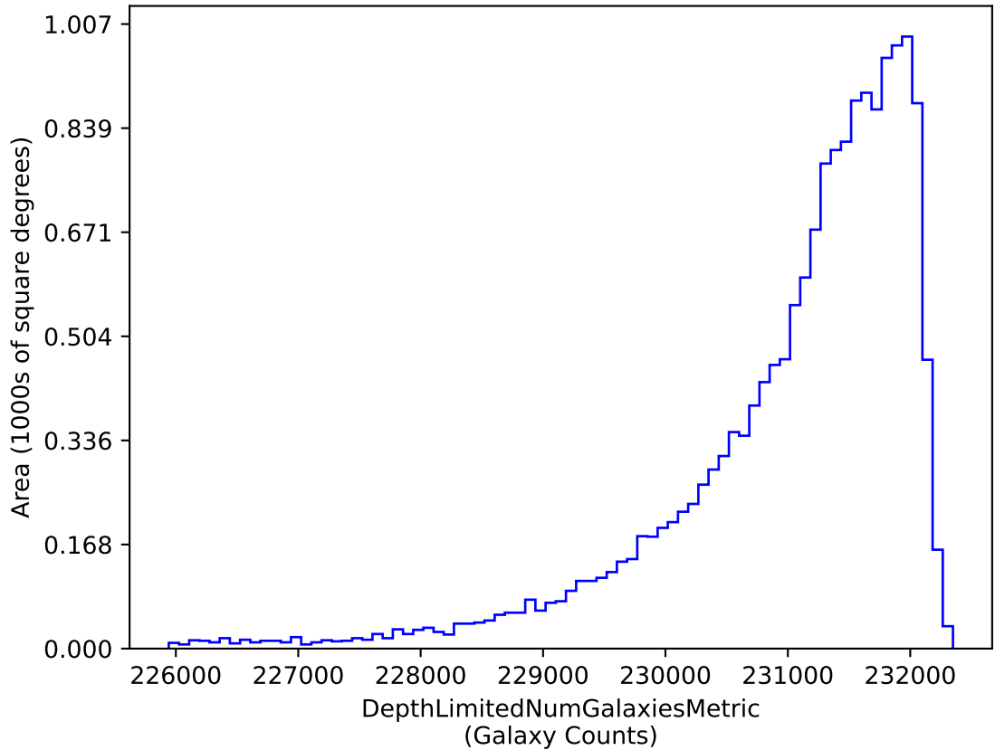
ddf_loaded_half_fl1_v3.4_10yrs i band galaxies non-DD: DepthLimitedNumGalaxiesMetric
