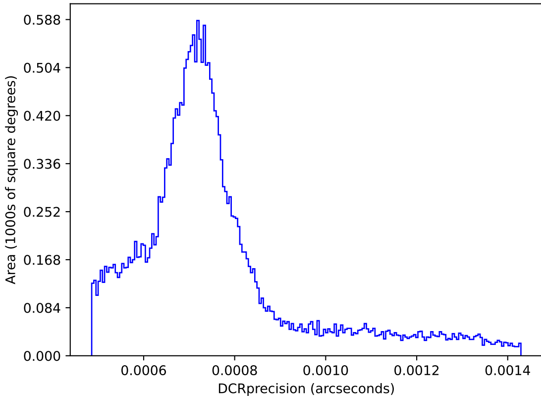
ddf_loaded_half_fl1_v3.4_10yrs : DCRprecision
