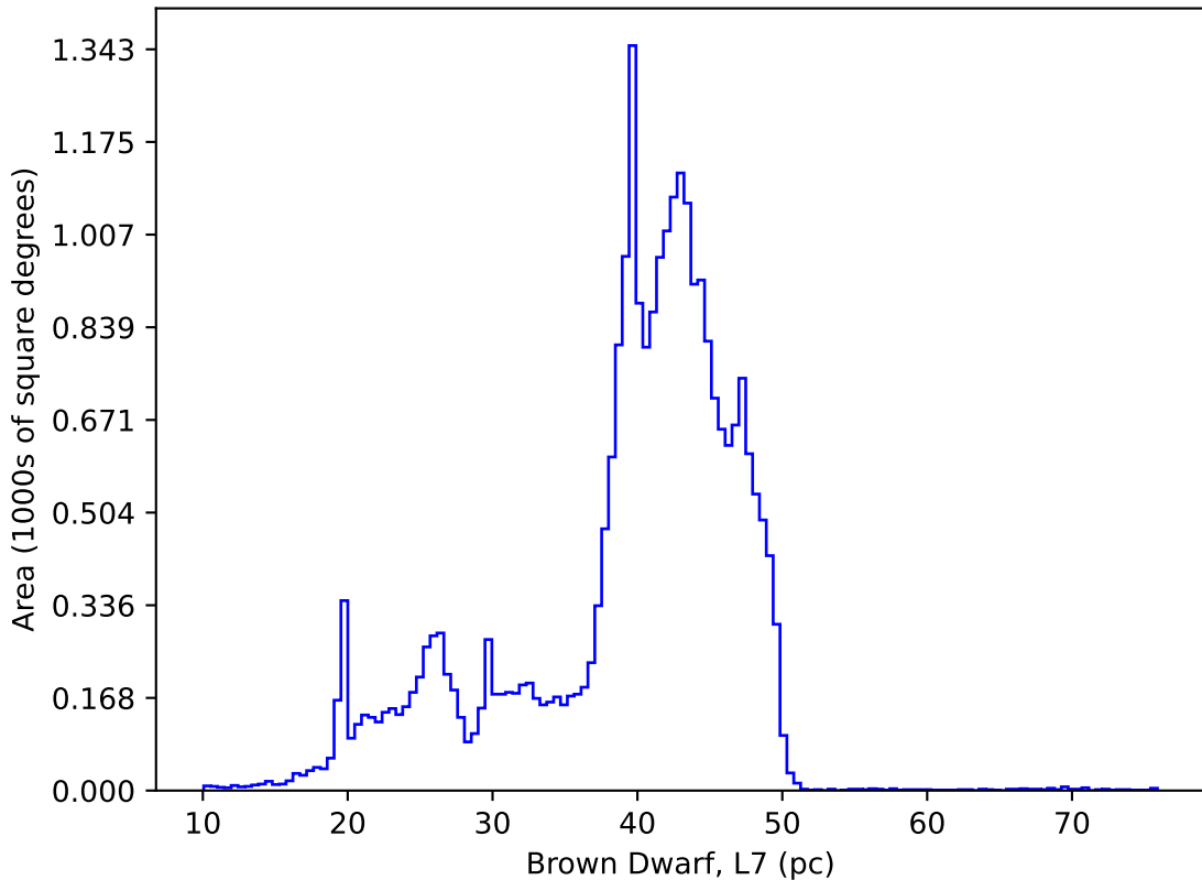
ddf_loaded_half_fl1_v3.4_10yrs : Brown Dwarf, L7
