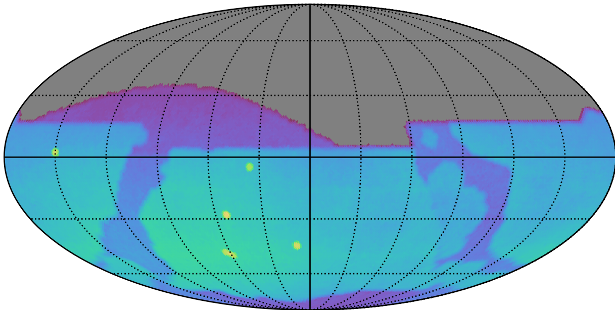
ddf_loaded_half_fl1_v3.4_10yrs : Brown Dwarf, L4
